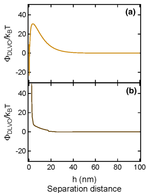
Fig. 4 Predicted normalized \Phi_{DLVO} interaction energy profiles for: a hAdV35–glass beads treated as sphere–plate, and b hAdV35–hAdV35 treated as sphere–sphere, as a function of separation distance (Here I_s = 1.4 mM, and pH 7.6)
